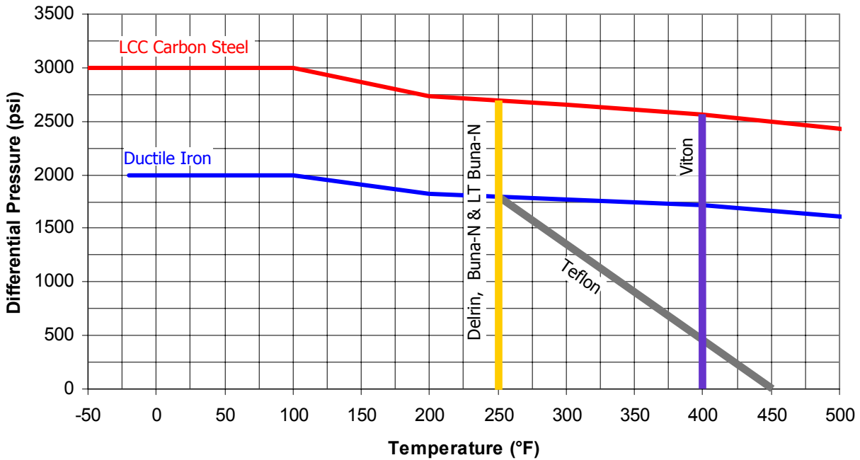
Pressure-Temperature Chart
