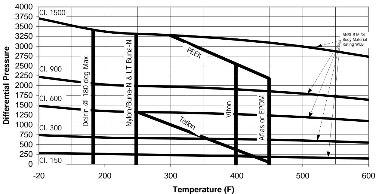
Pressure Temp Chart
